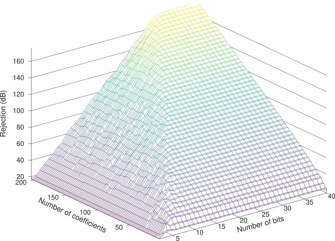
Mean rejection as a function of number of coefficients and number of bits
