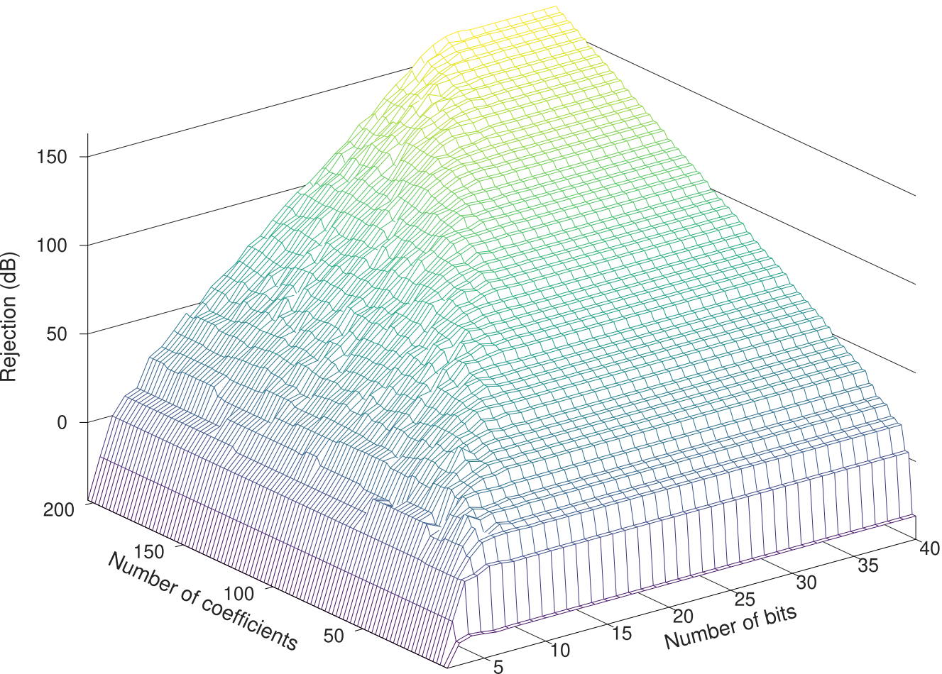
Custom criterion of rejection as a function of number of coefficients and number of bits
