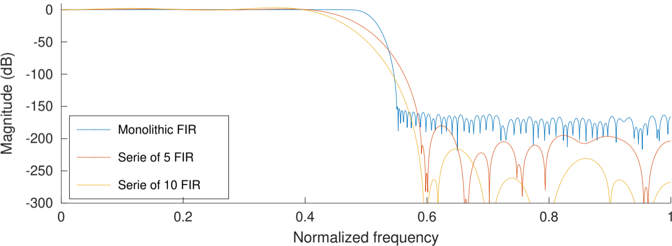
Comparison between a series of FIR and a monolithic FIR
