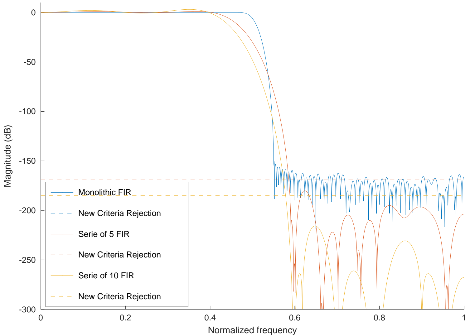
Comparison between a series of FIR and a monolithic FIR
